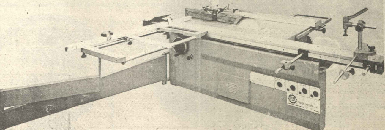
Teno squadatrice Tenoning-sawing machine Zapfen-Kreisägemaschine Teno scie circolare Teno-Sierra circular
